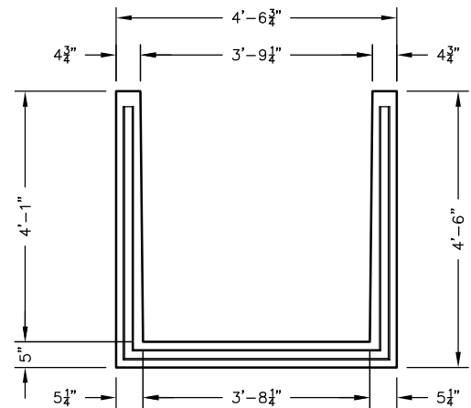
END VIEW - BASE
