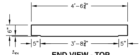
END VIEW - TOP
