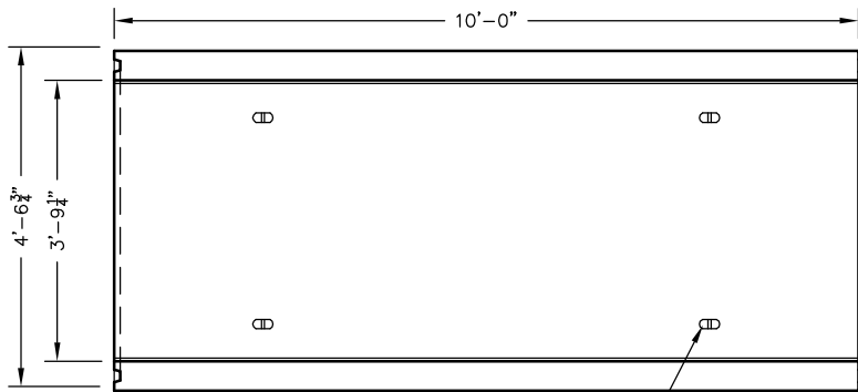
PLAN VIEW - BASE
